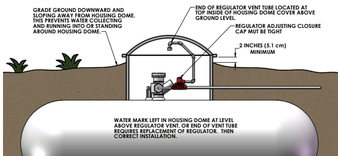
Figure 5: Underground Installation
